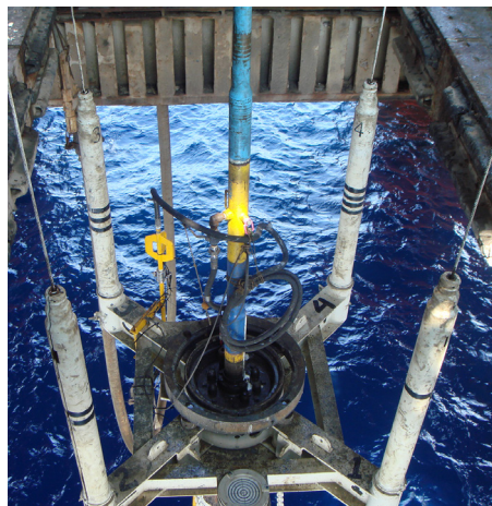
CEMENT TOP-UP SYSTEMS
