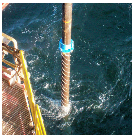
JACK-UP HIGH PRESSURE RISER ANALYSIS
