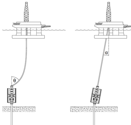
SEMI-SEB/DRILL SHIP RISER ANALYSIS
