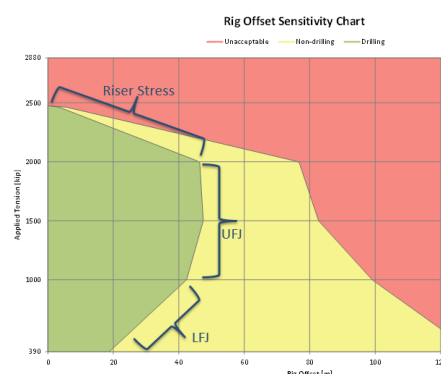
SEMI-SUB/DRILL SHIP RISER ANALYSIS
